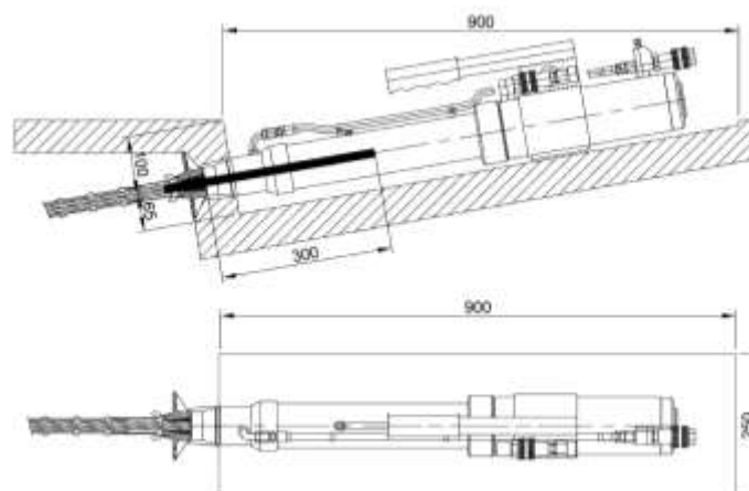
Figure 90 Clearance requirements with jack Alevin A7-24
