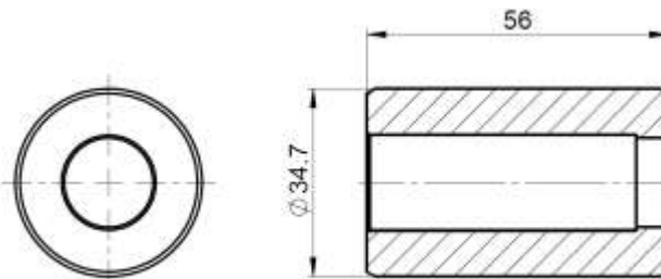
Figure 2 Compression fitting CFE6
