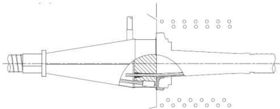
Coupler type K with anchorage type GC
