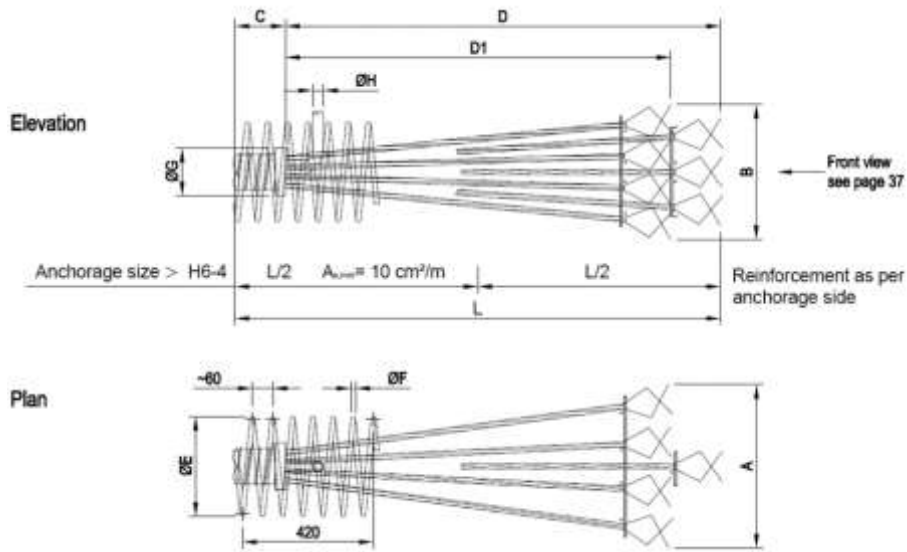
Figure 48 Anchorage and local anchorage reinforcement type H @ 28/35 MPa
