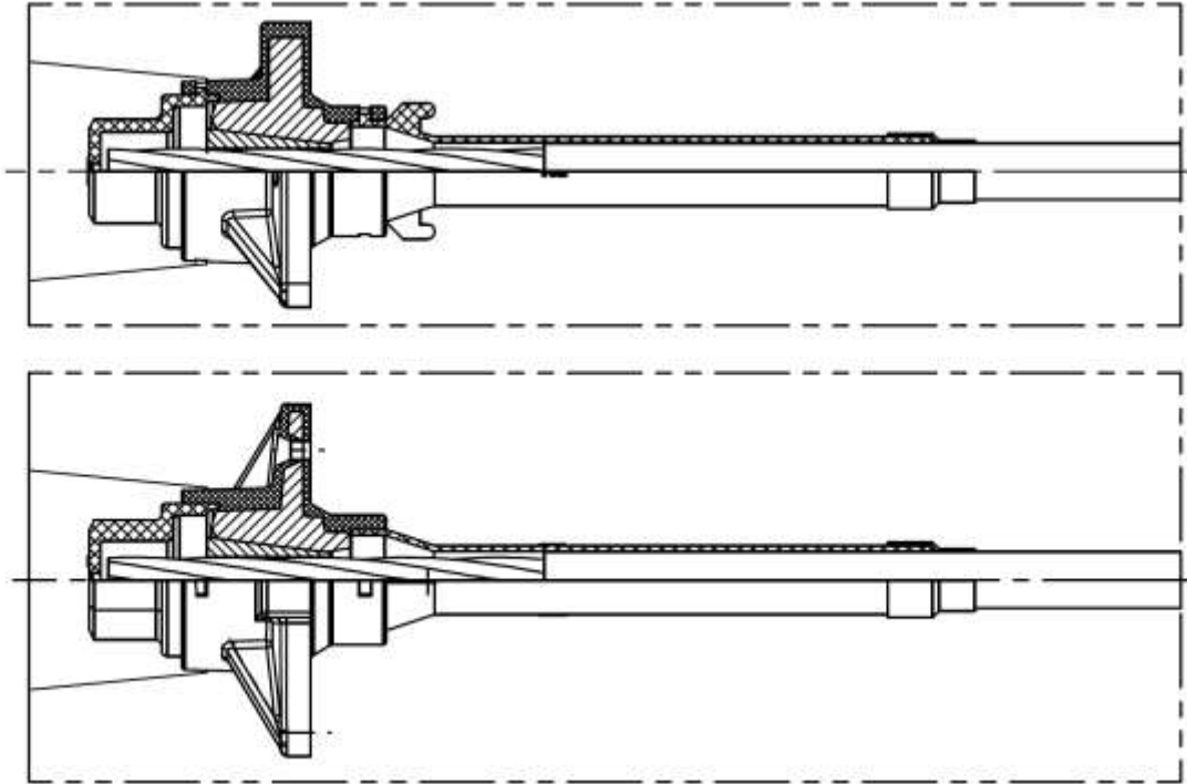
Figure 65 Anchorage type S 6-1 PLUS - Unbonded system
