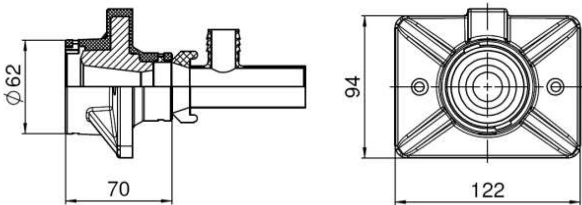
Figure 67 Anchorages type S 6-1 PLUS - Dimensions
