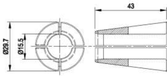
Figure 58 Wedge W6N
