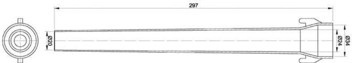
Figure 72 Sleeve S 6-1 Standard (for unbonded application)
