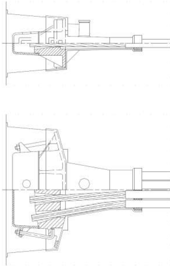
Figure 76 Anchorage type S 6-4 - Unbonded system
