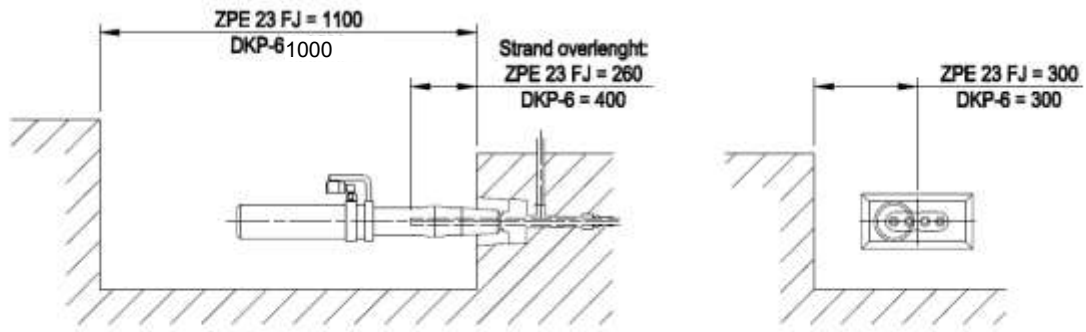
Figure 88 Clearance requirements with jacks DKP-6 and ZPE 23FJ
