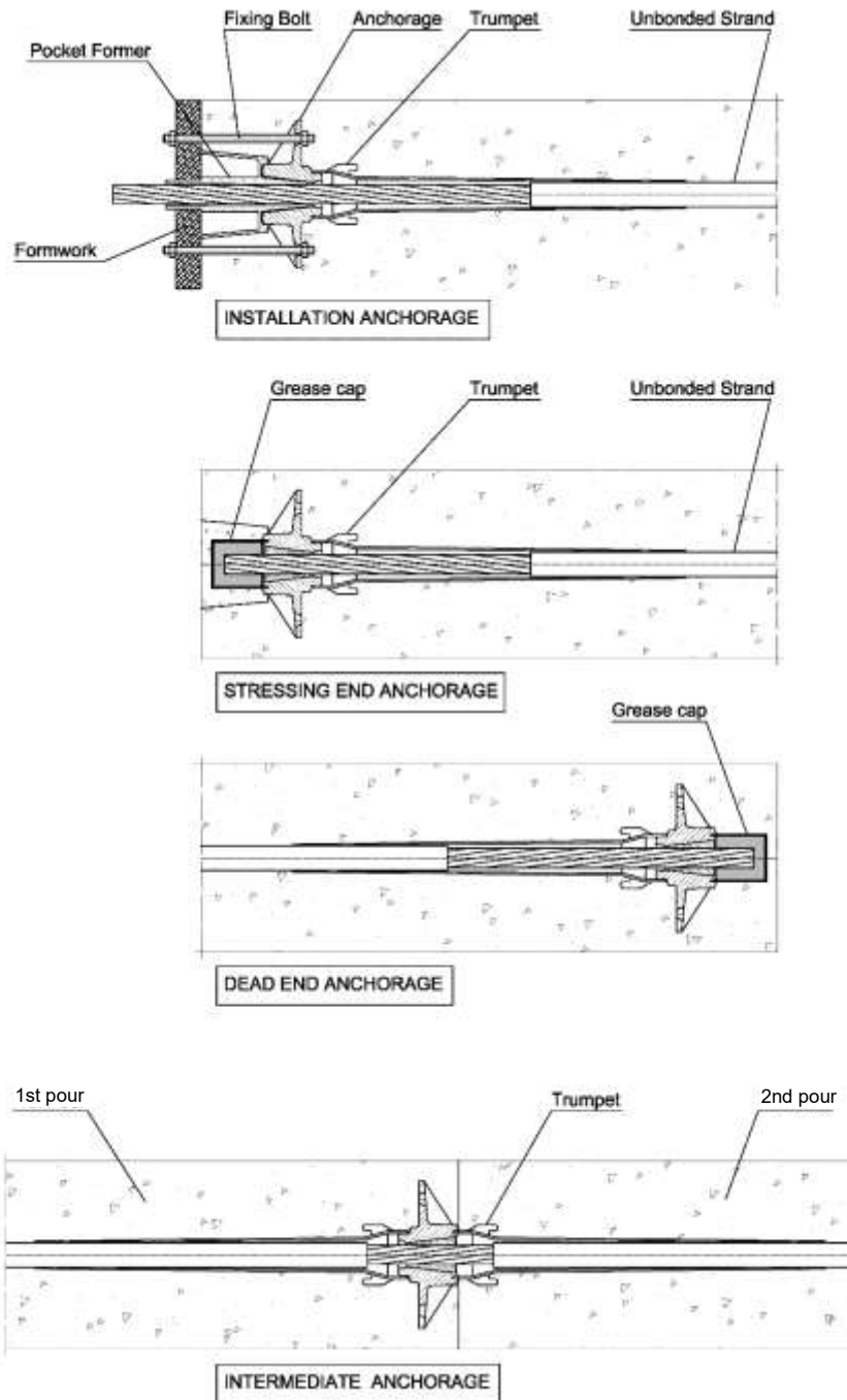
Figure 69 Anchorages type S 6-1 Standard - Unbonded system
