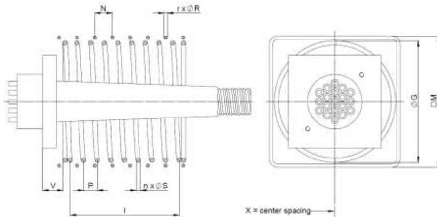
Figure 31 Local anchorage zone reinforcement type E @ 32/40 MPa
