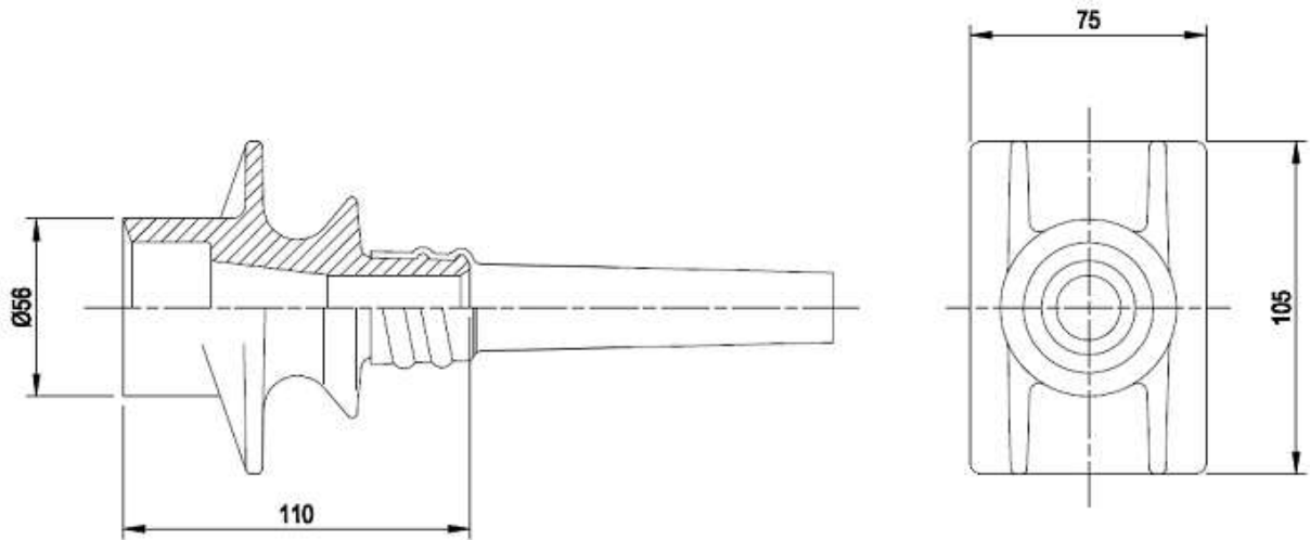
Figure 63 Anchorage type S 6-1 - Dimensions
