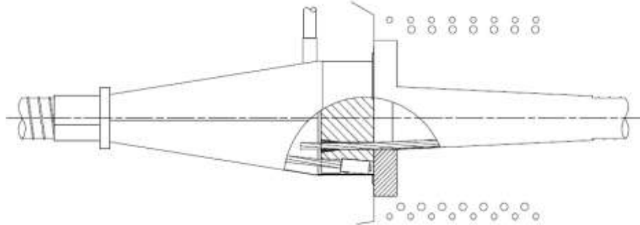
Coupler type K with anchorage type E
