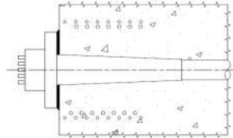
Anchorage placed against concrete structure
