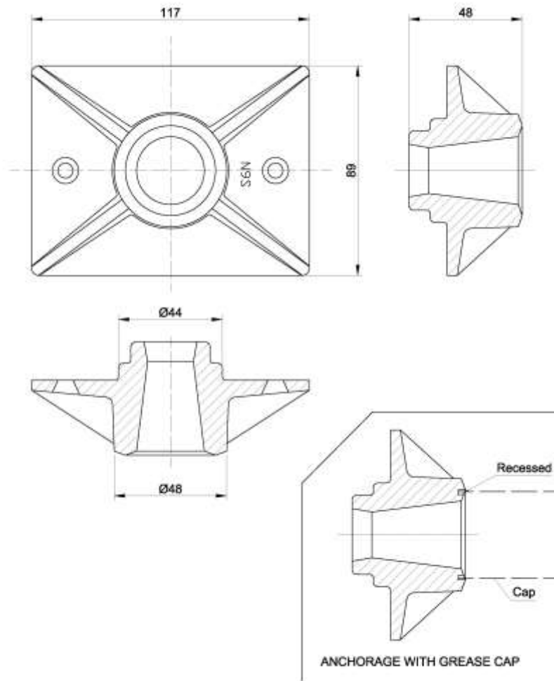
Figure 71 Anchorage body type S 6-1 Standard
