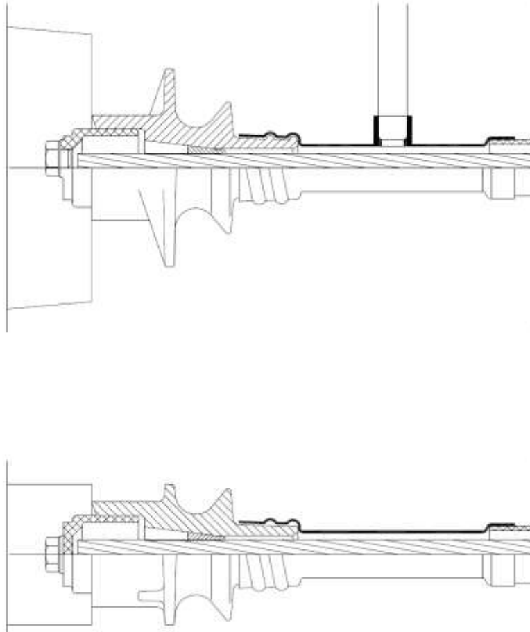
Figure 62 Anchorage type S 6-1 - Bonded system
