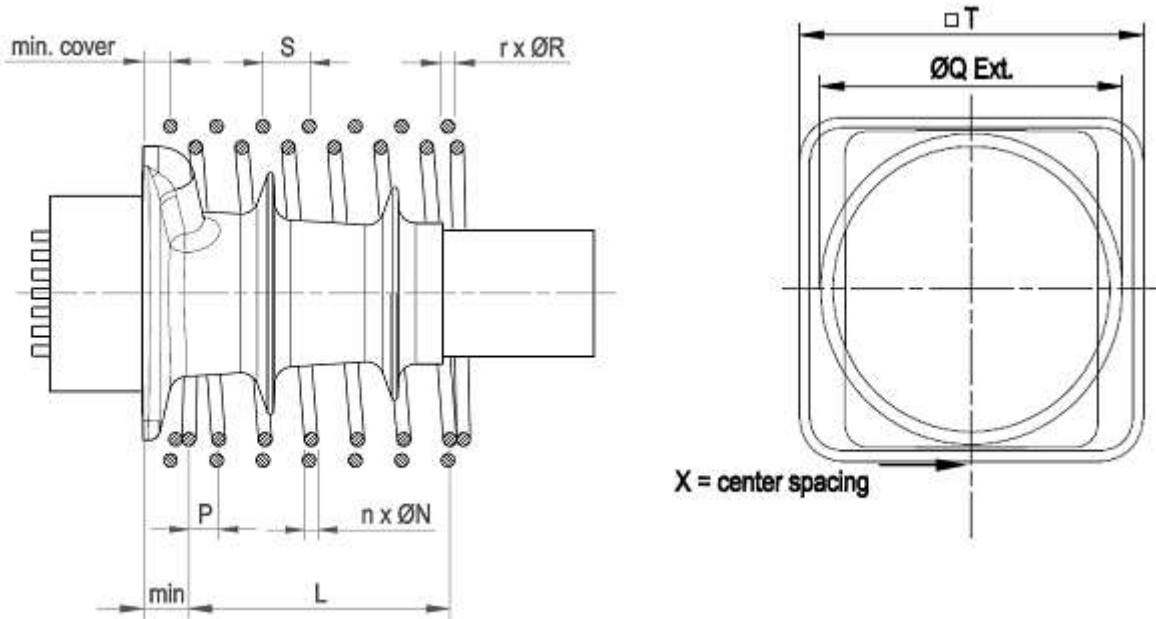
Figure 47 Local anchorage zone reinforcement type NC and NC-U @ 53/64 MPa
