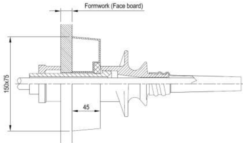
Figure 64 Anchorage type S 6-1 – Dimension of placing devices
