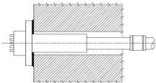
Figure 13 Categories of use and arrangements of anchorages type E
