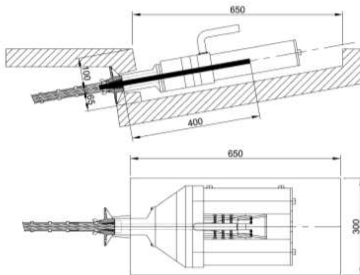
Figure 89 Clearance requirements with Twin jack 25T
