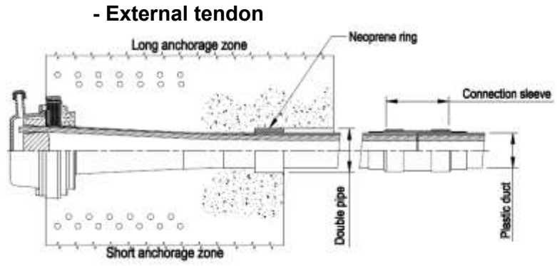
Figure 35 Arrangements anchorage type CS external tendon
