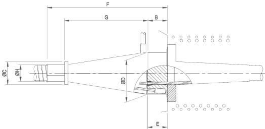
Figure 50 Couplers type K dimensions
