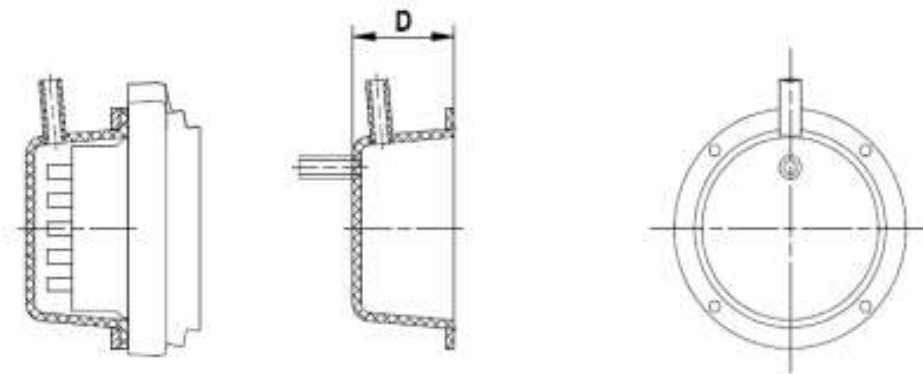
Figure 12 Permanent polymeric caps for anchorage type CS
