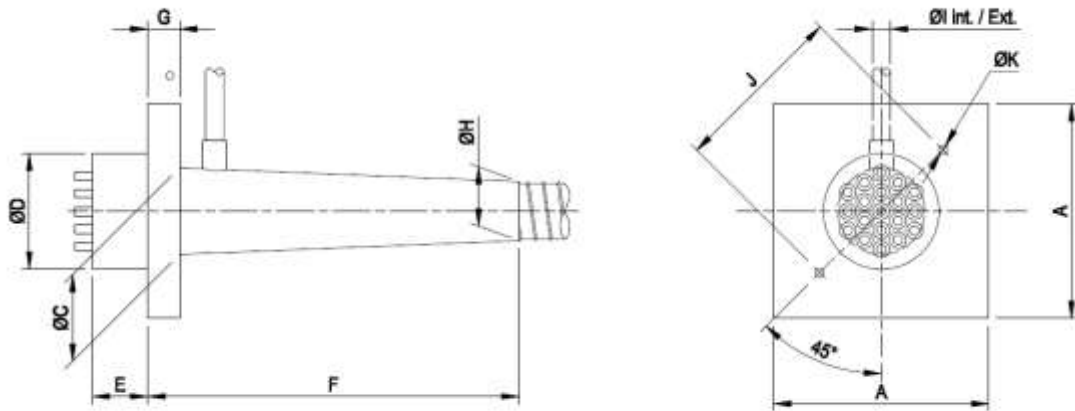
Figure 22 Anchorages type E @ 23/28 and 28/35 MPa dimensions
