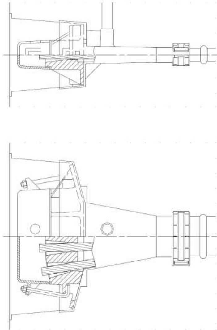
Figure 77 Anchorage type S 6-4 - Bonded system
