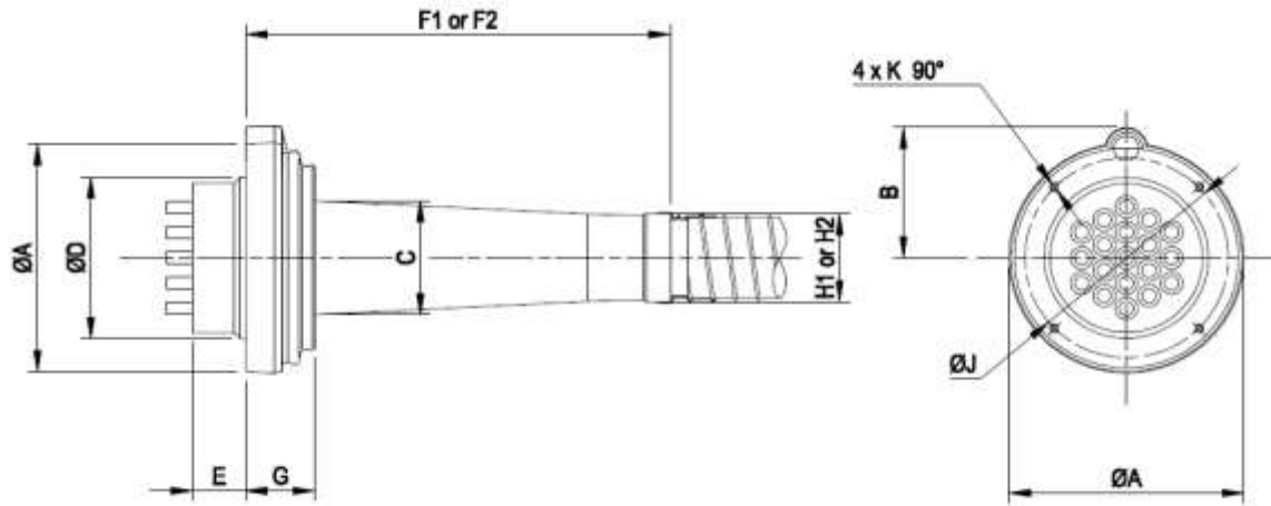
Figure 36 Anchorages type CS @28/35 MPa dimensions
