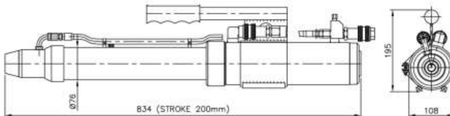
Figure 87 Stressing jack Alevin A7/24
