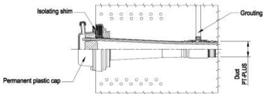
Figure 34 Arrangements anchorage type CS cast in concrete structure
