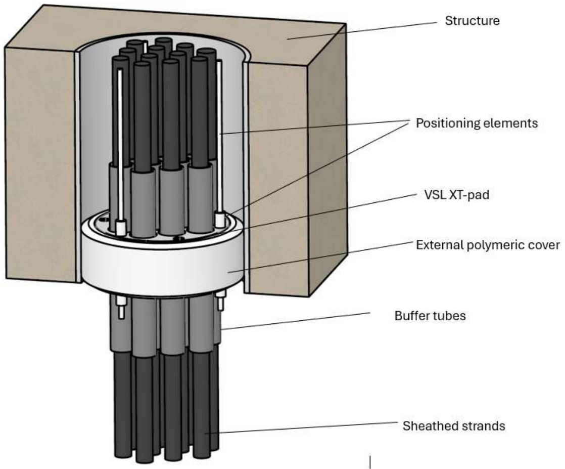
Figure 21 XT-deviator – Arrangement inside guide tube
