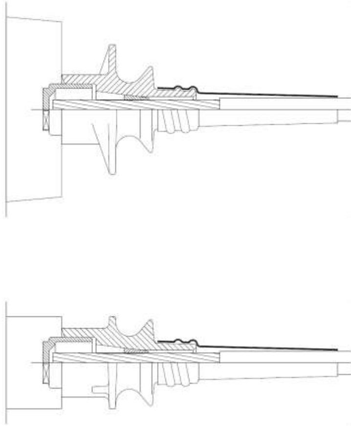
Figure 61 Anchorage type S 6-1 - Unbonded system
