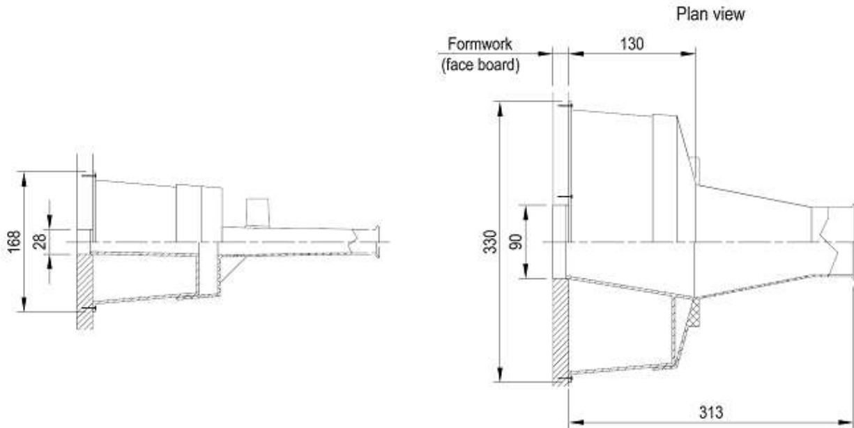
Figure 78 Anchorages type S 6-4 - Body and sleeve dimensions
