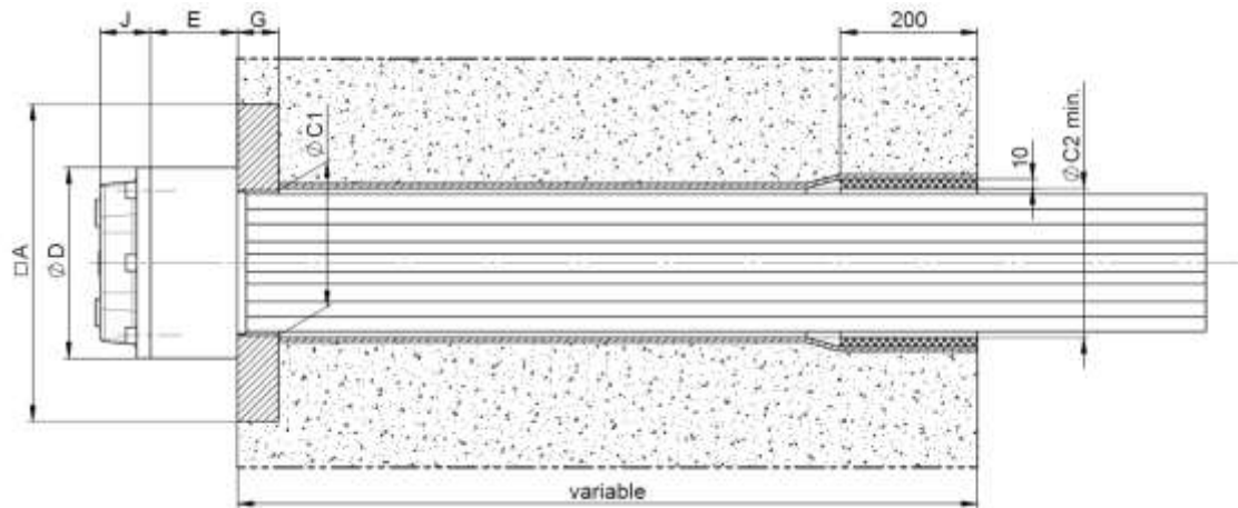
Figure 25 Anchorage type E-WTe - Arrangement without shim plate - Dimensions
