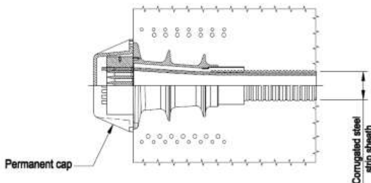
Figure 44 Categories of use arrangements anchorage type NC and NC-U
