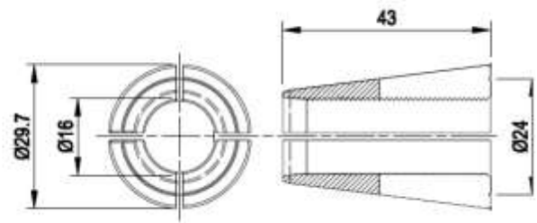
Wedge W6S
