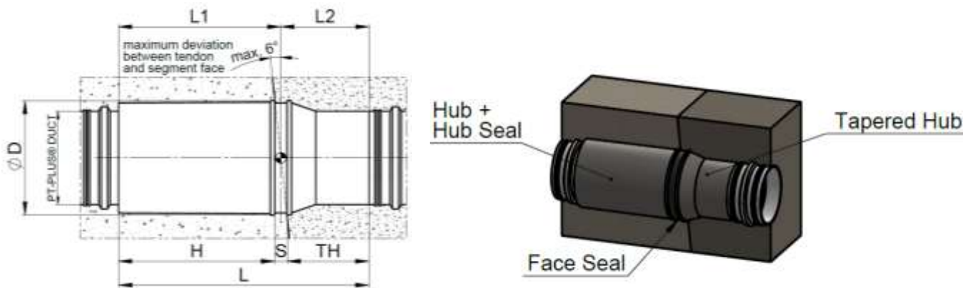
Figure 57 Segmental Couplers – PT-Plus Round Duct
