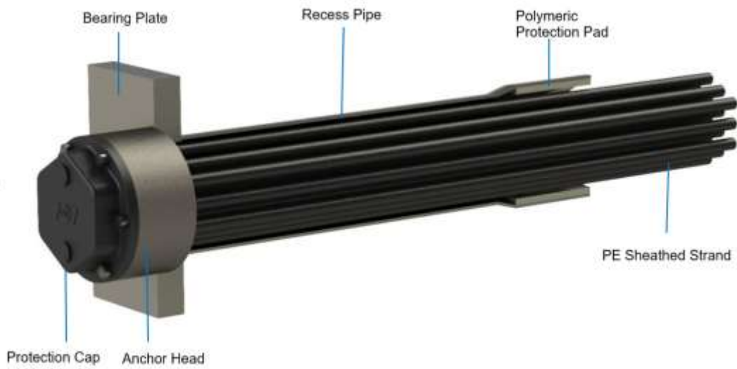
Figure 14 Anchorages type E-WTe (External unbonded tendons)- Arrangement without shim plate
