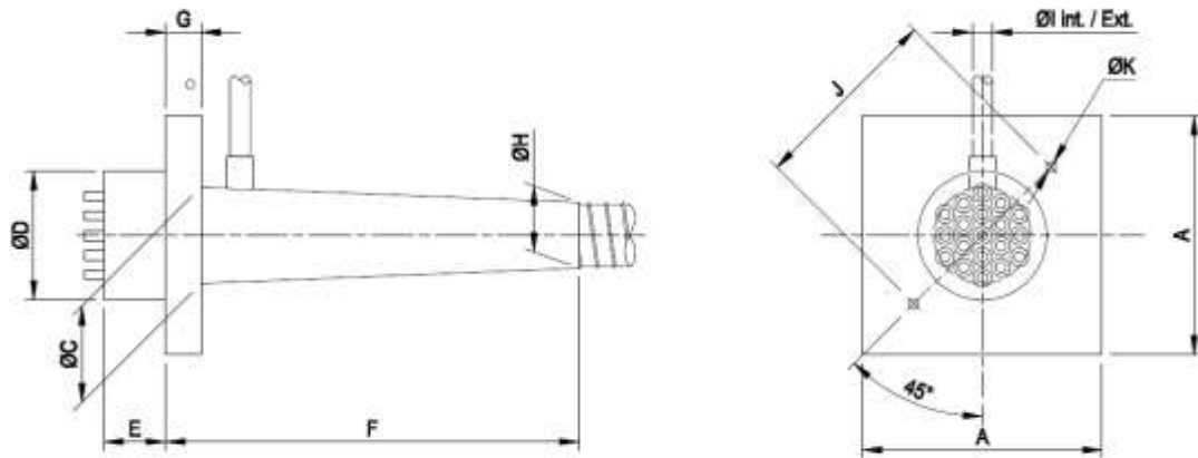
Figure 24 Anchorages type E @ 43/53 MPa dimensions
