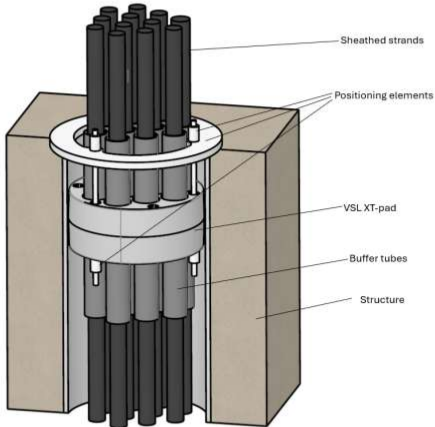
Figure 19 XT-deviator – Arrangement at the exit of guide tube
