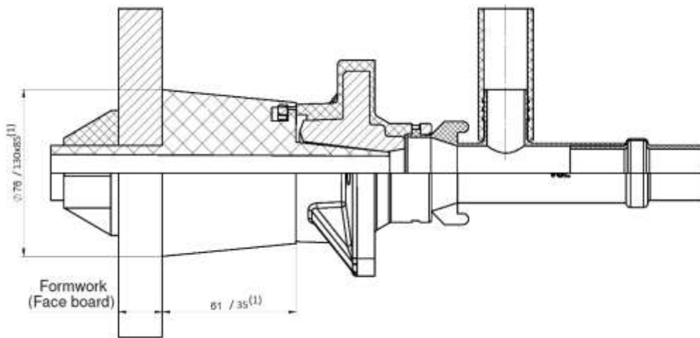
Figure 68 Anchorages type S 6-1 PLUS – Dimensions of placing devices
