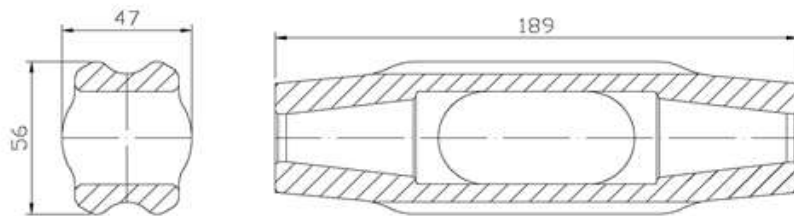
Figure 74 SK 6-1 SL Spring loaded coupler body dimensions
