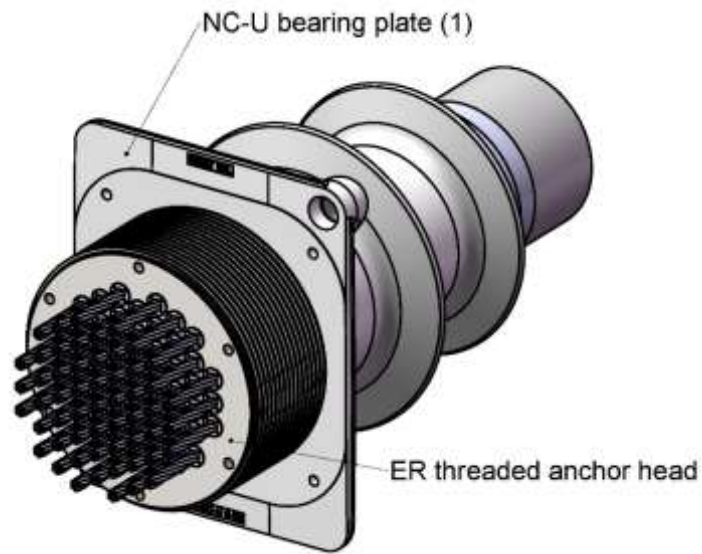
Figure 45 Assembly with threaded anchor head for load monitoring
