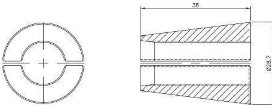
Figure 59 Wedge W6M (for use with T15.2 strand)
