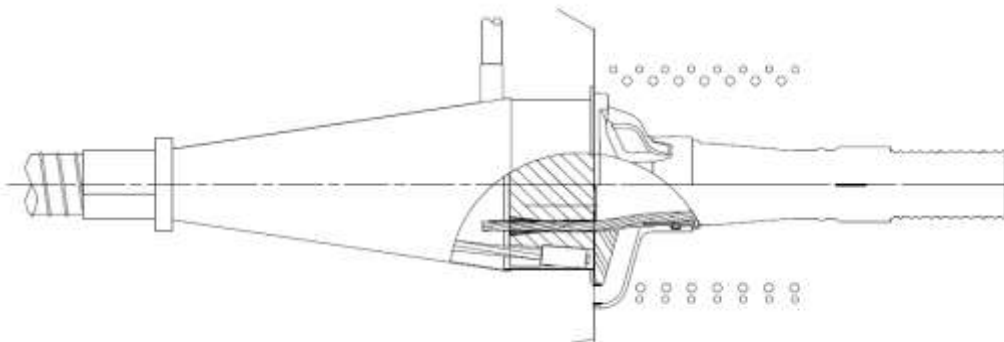
Figure 49 Categories of use arrangements couplers type K
