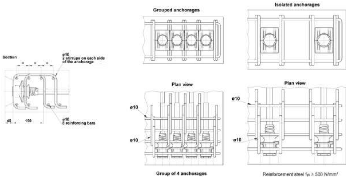
Figure 80 Example of additional reinforcement to combine with main one type S 6-1 f_{c,min}(t) > 16/20 \text{ N/mm}^2
