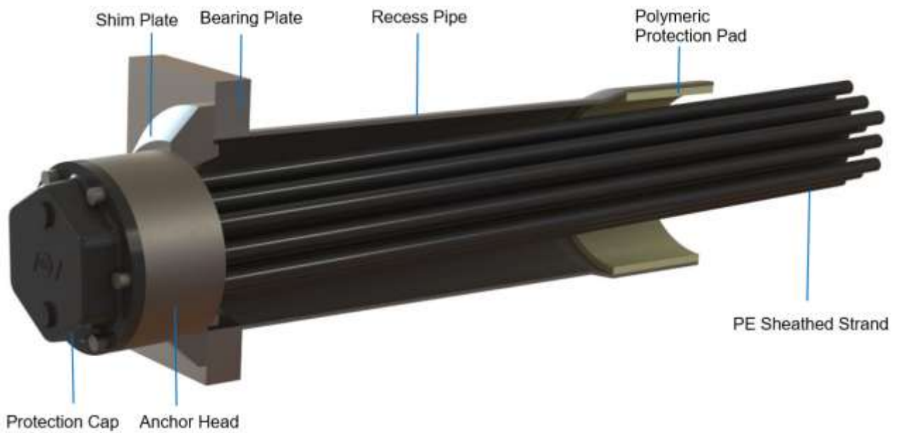
Figure 15 Anchorages type E-WTe (External unbonded tendons)- Arrangement with shim plate
