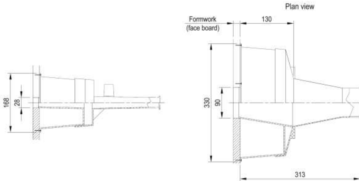
Figure 79 Anchorages type S 6-4 – Dimensions of placing devices
