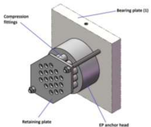
Figure 13 Categories of use and arrangements of anchorages type E
