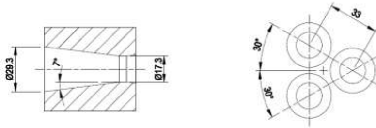
Figure 5 Hole detail anchor head type E
