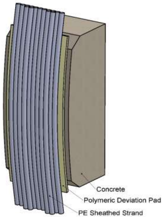
Figure 17 Deviator E-WTe- Curved deviator
