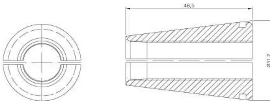
Figure 60 Wedge W6ML (for use with spring-loaded coupler)
