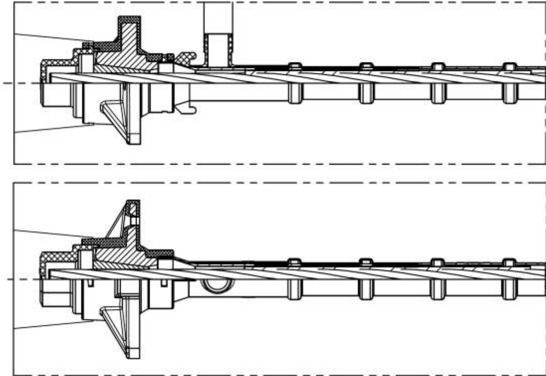
Figure 66 Anchorage type S 6-1 PLUS - Bonded system
