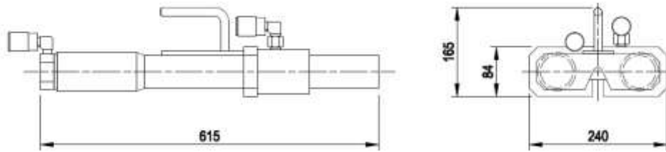
Figure 84 Stressing jack DKP-6
