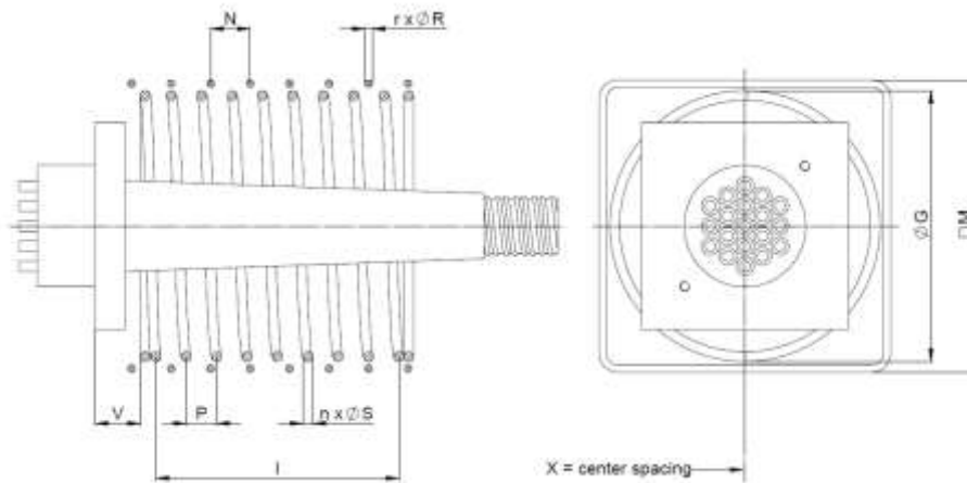
Figure 30 Local anchorage zone reinforcement type E @ 28/35 MPa
