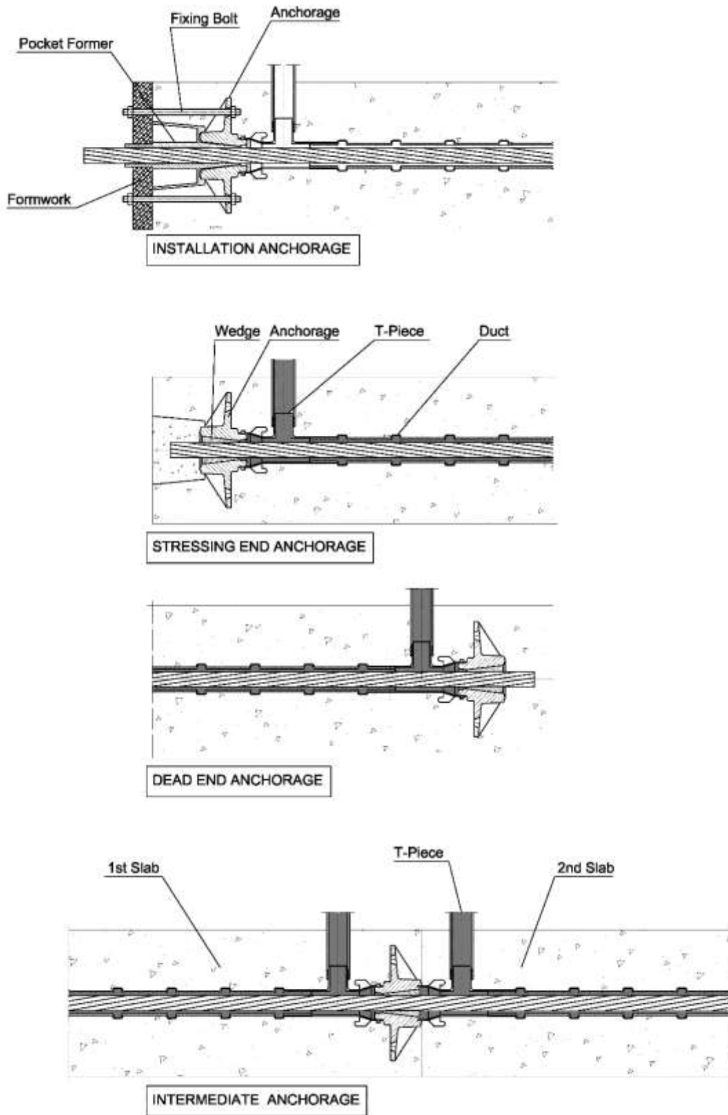
Figure 70 Anchorage type S 6-1 Standard - Bonded system
