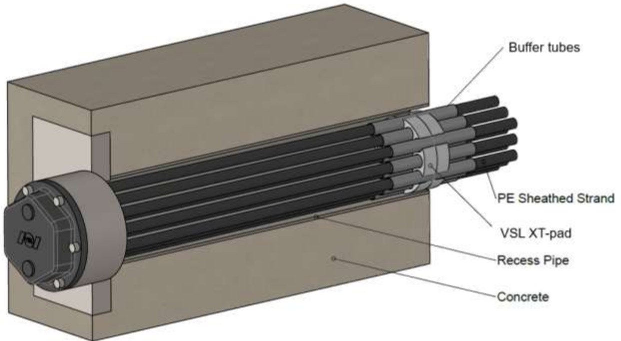
Figure 18 XT-deviator based on XT-pads
