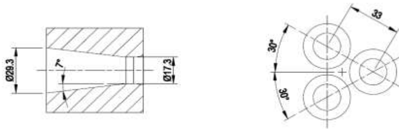
Figure 8 Hole detail anchor head type CS
