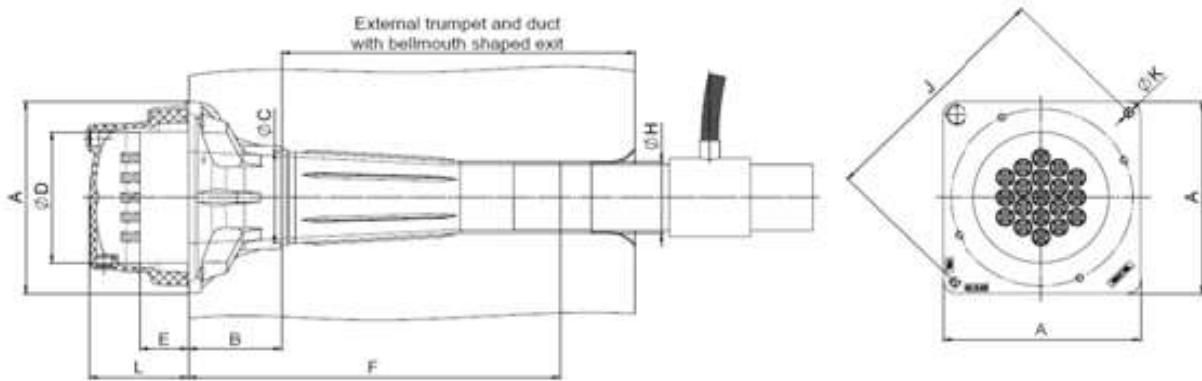
Figure 40 Anchorages type GC external tendons dimensions
