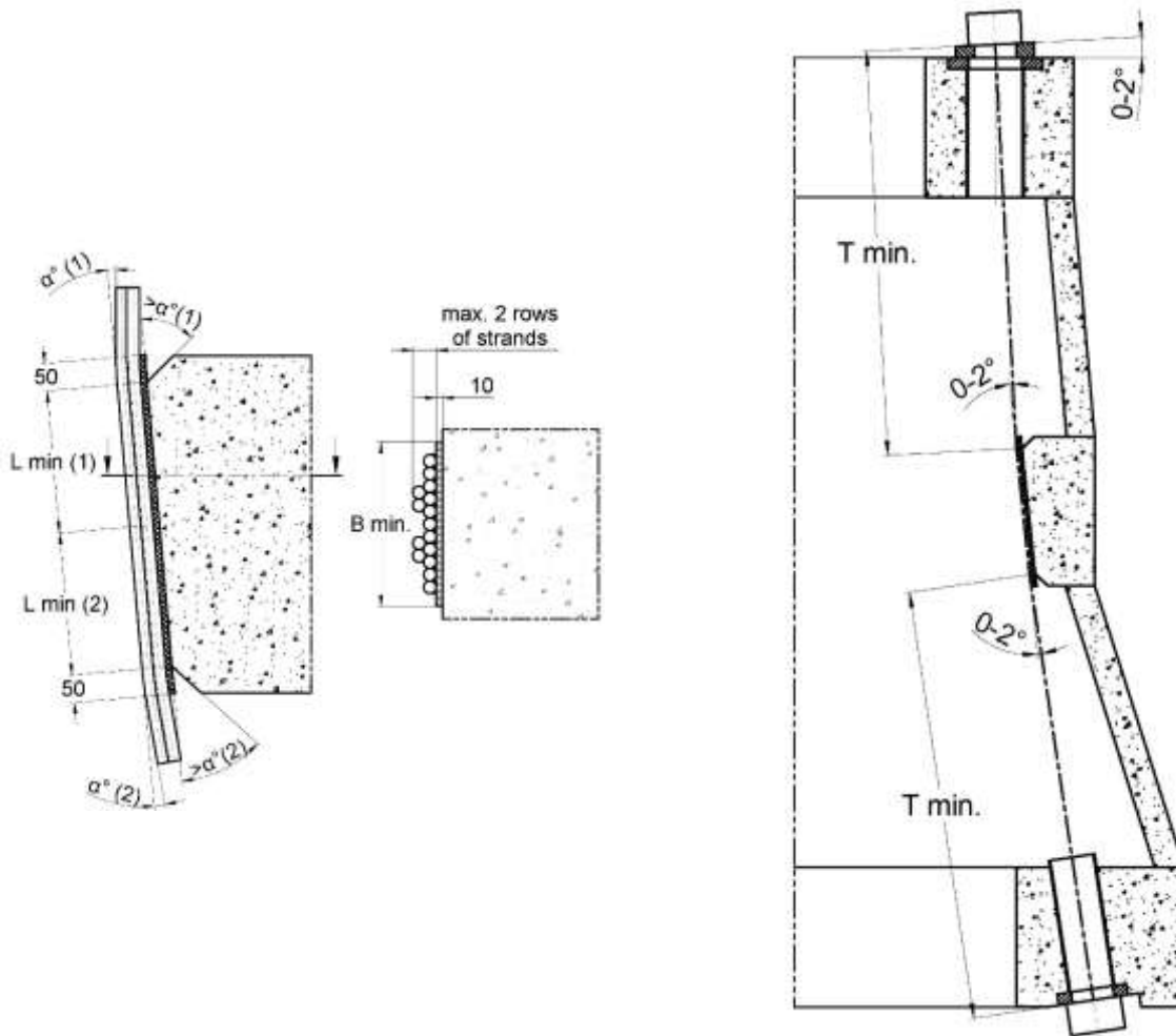
Figure 27 Deviator E-WTe – Flat deviator - Geometry and dimensions
