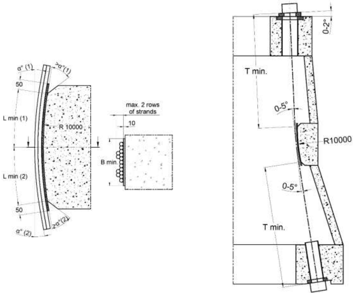
Figure 28 Deviator E-WTe – Curved deviator - Geometry and dimensions
