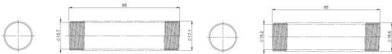
Figure 3 Insert CF6
