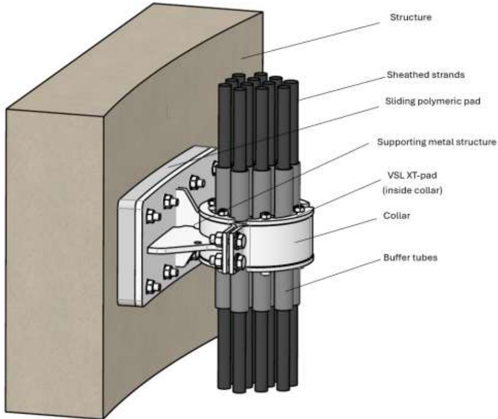
Figure 20 XT-deviator – Arrangement at mid length of the tendon
