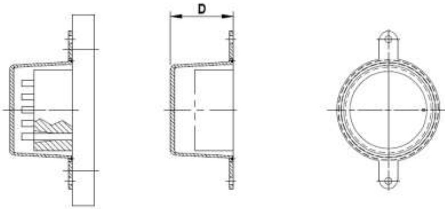
Figure 11 Permanent steel caps for anchorage type GC, E, NC, NC-U
