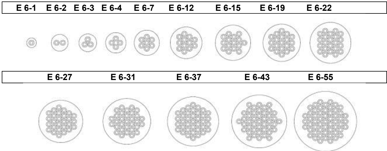
Figure 6 Hole spacing anchor head type E
