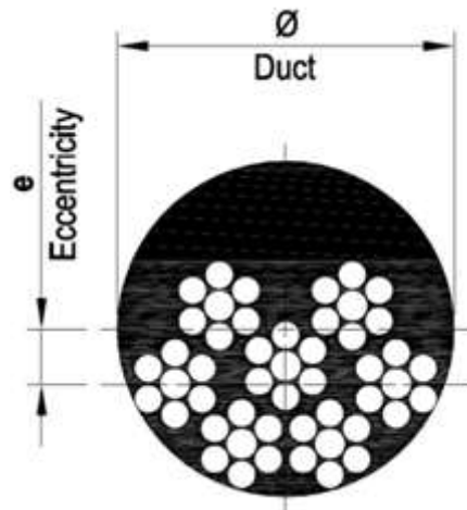
Figure 56 Ducting dimensions
