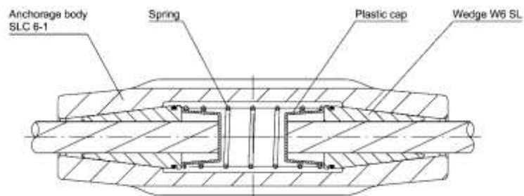
Figure 75 SK 6-1 SL Spring loaded coupler assembly drawing
