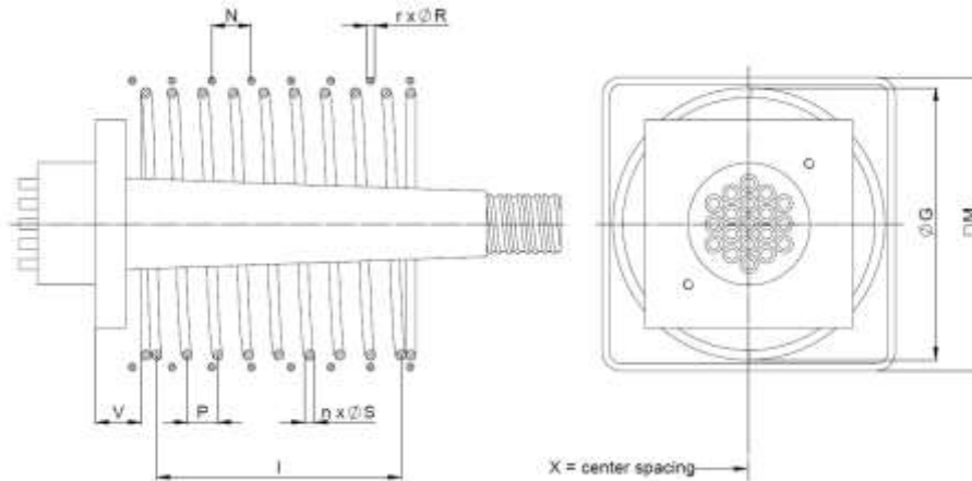
Figure 32 Local anchorage zone reinforcement type E @ 36/45 MPa
