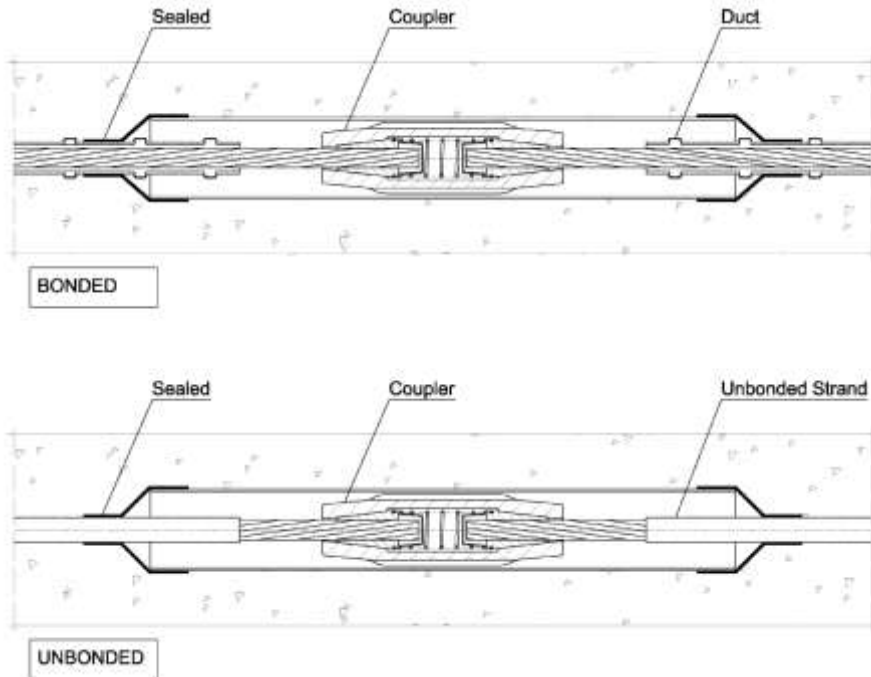
Figure 73 SK 6-1 SL Spring loaded coupler ( bonded and unbonded application )
