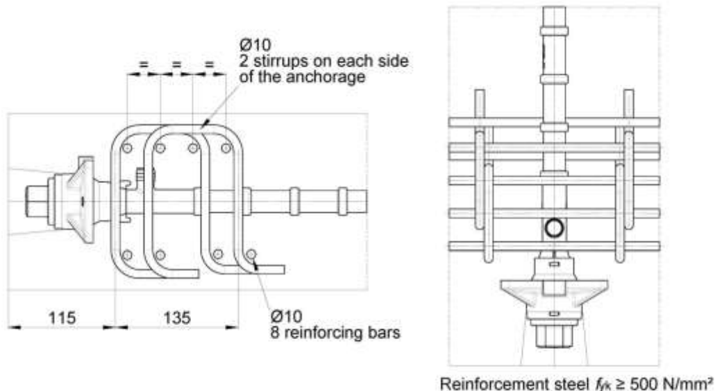
Figure 81 Example of additional reinforcement to combine with main one type S 6-1 PLUS and S 6-1 Standard f_{c,min}(t) > 16/20 \text{ N/mm}^2
