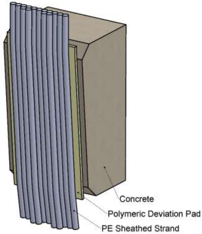
Figure 16 Deviator E-WTe – Flat deviator
