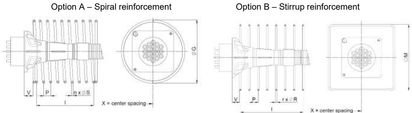
Figure 43 Local anchorage zone reinforcement type GC external and electrically isolated tendons
