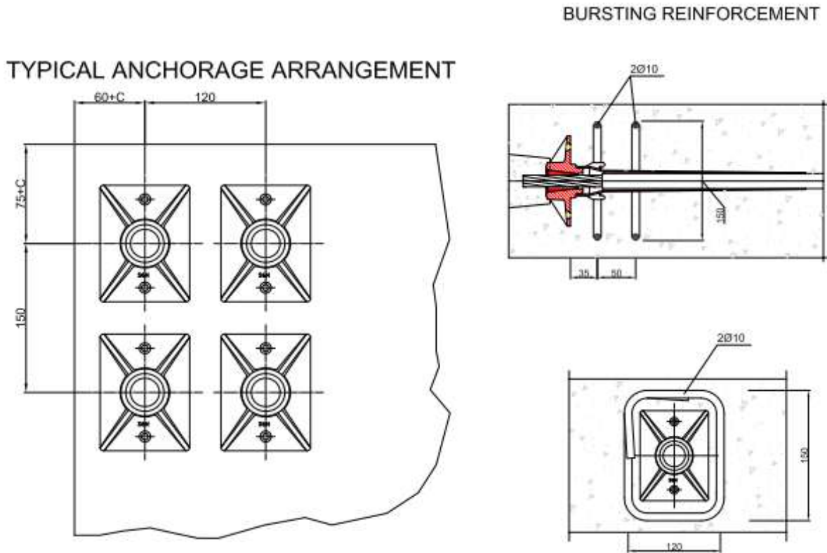
Figure 82 Example of additional reinforcement to combine with main one type S 6-1 PLUS and S 6-1 Standard f_{c,min}(t) > 20/25 \text{ N/mm}^2
