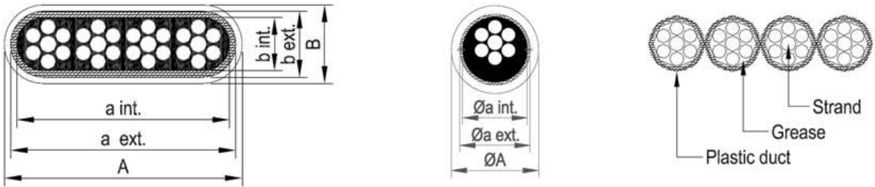
Figure 91 VSL PT-PLUS® Duct bonded / bonded / unbonded
