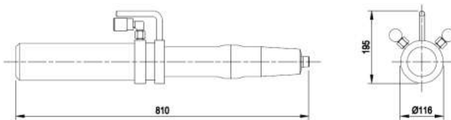
Figure 86 Stressing jack ZPE-23FJ
