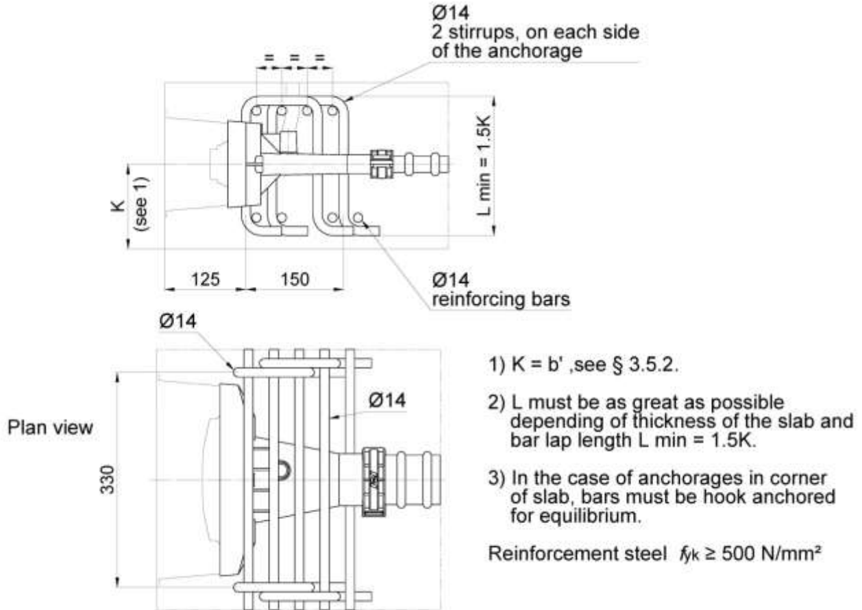
Figure 83 Example of additional reinforcement to combine with main one type S 6-4 f_{c,min}(t) > 16/20 \text{ N/mm}^2
