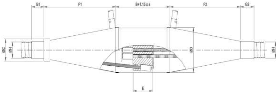
Figure 52 Couplers type V dimensions
