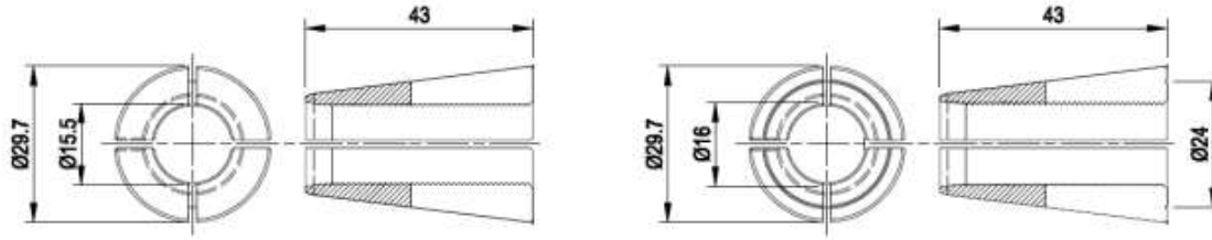
Figure 1 Wedge W6N
