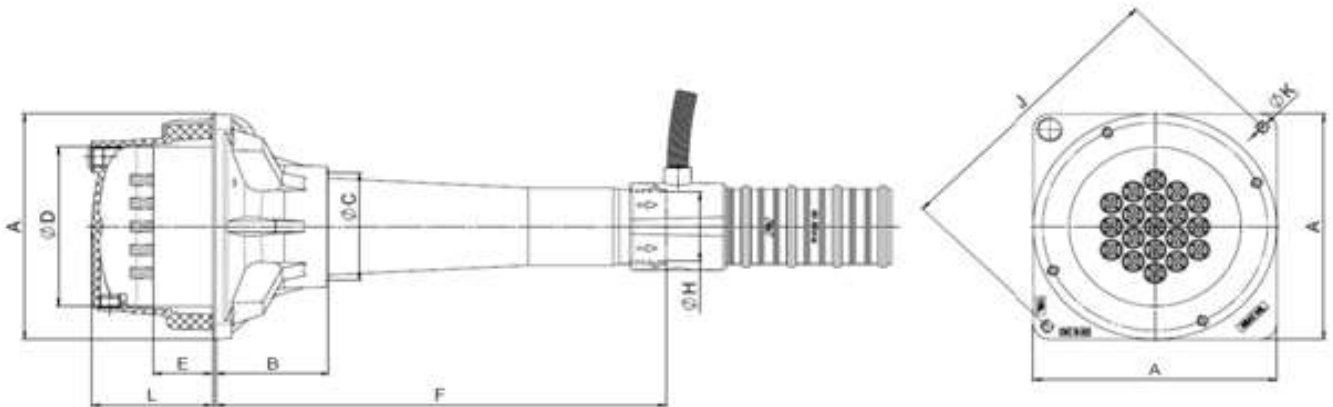
Figure 41 Anchorages type GC electrically isolated tendons dimensions
