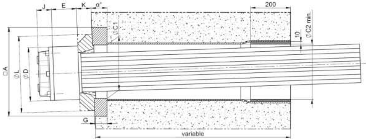
Figure 26 Anchorage type E-WTe - Arrangement with shim plate - Dimensions
