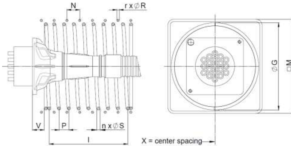
Figure 42 Local anchorage zone reinforcement type GC internal bonded post-tensioning
