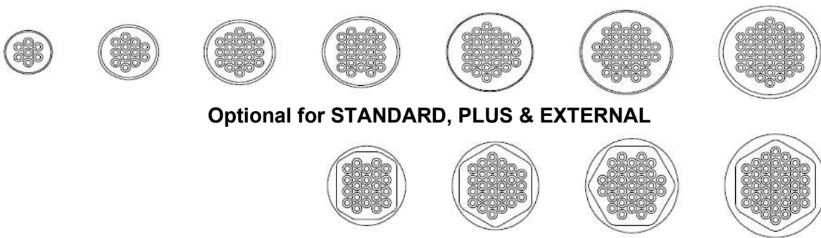
Figure 9 Hole spacing anchor head type CS
