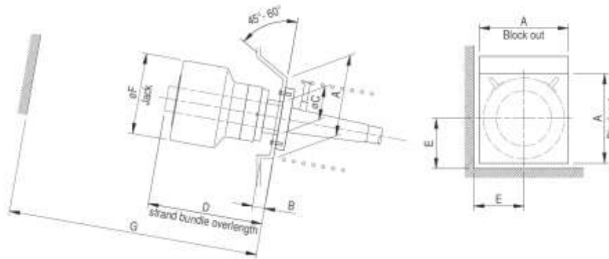
Figure 53 Block-out dimensions – Clearance requirements
