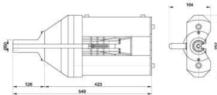
Figure 85 Twin jack 25T
