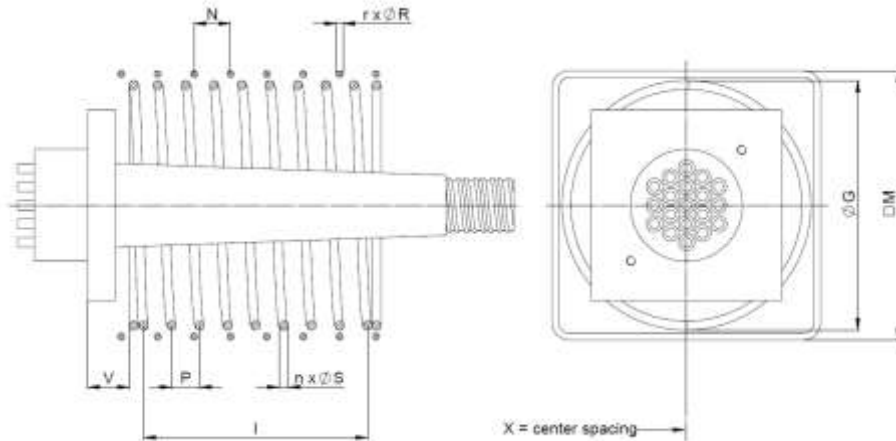
Figure 33 Local anchorage zone reinforcement type E @ 43/53 MPa
